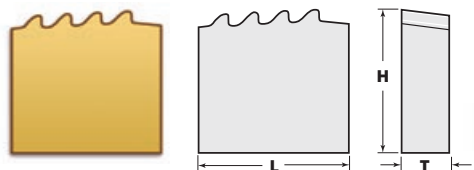
8045E (4T-8P-IMPROVED BUTTRESS-EXT)
