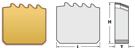
8045I (4T-8P-IMPROVED BUTTRESS-INT)
