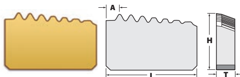
807 (7T-8RD-INT)
