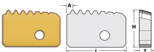
814 (4T-8RD-INT)
