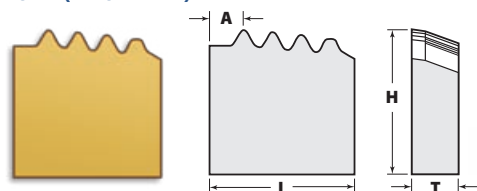
814 (4T-8RD-INT)
