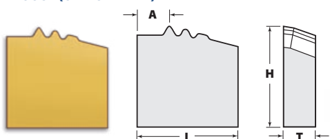
1003I (3T-10RD-INT)
