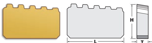
15BTI (5T-5P-1" BUTTRESS-INT)
