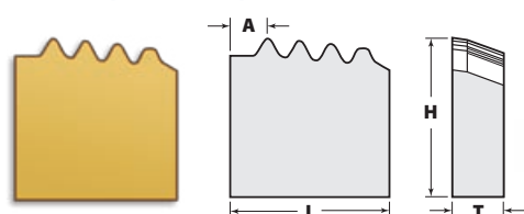
814-JH (4T-8RD-INT)
