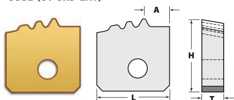
833E (3T-8RD-EXT)
