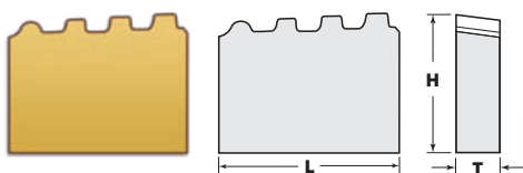
55P75E (5T-5P-3/4" BUTTRESS-EXT)
